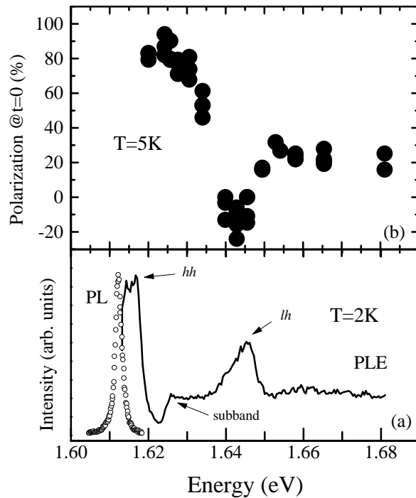
Figure 2. (a) Photoluminescence (open points) and excitation spectra (curve) of a 77 Å wide GaAs quantum well recorded at 2 K under an excitation of 5 \text{ mW cm}^{-2} . The peaks are the heavy-hole (hh) and light-hole (lh) excitons. The step corresponds to the hh subband continuum. (b) The initial degree of polarization as a function of excitation energy obtained from TR-PL experiments at 5 K.
